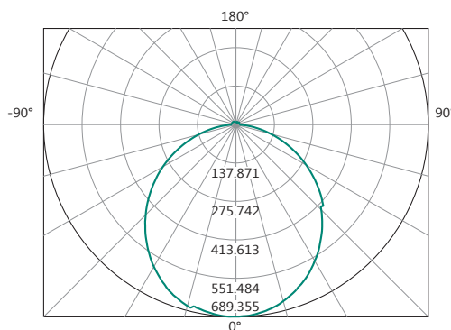
Polar Curve
