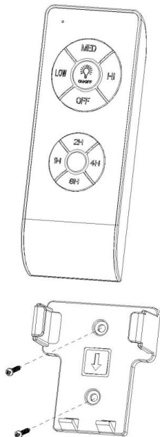
Installation of Transmitter Wall Mount Holder with two screws.
