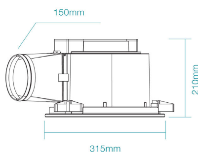
Round 295 / Square 295
