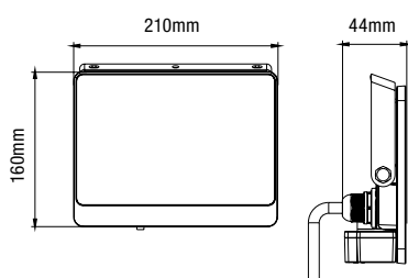
GUARD 30W
