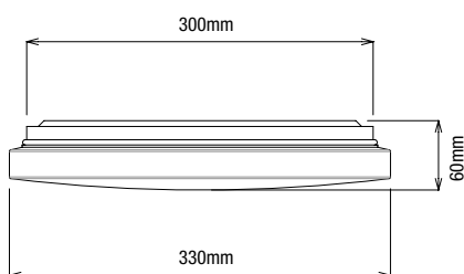
ORBIT 330MM
