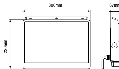
GUARD 100W
