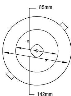
RECESSED
