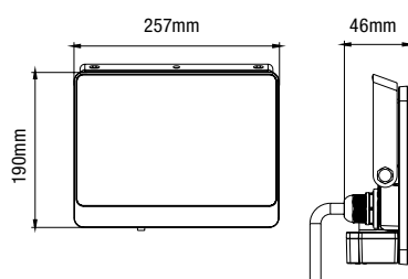
GUARD 50W
