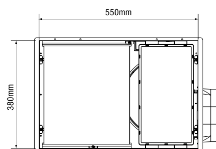
TOP VIEW ELEVATION
